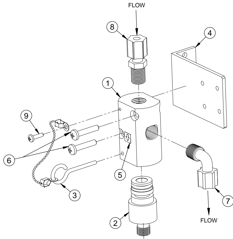
EXPLODED VIEW
