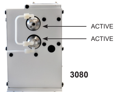
Single (or Dual) Sample, Dual Stage Thermoelectric Gas Cooler
